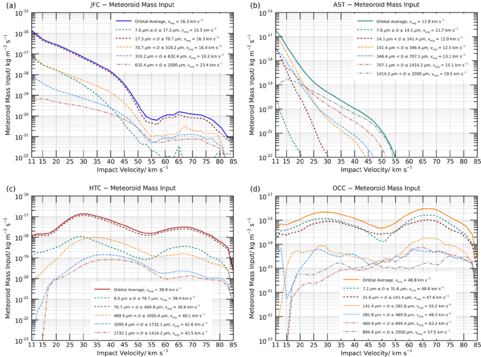
Figure 4. from Juan Diego Carrillo-Sánchez et al 2026 Planet. Sci. J. 7 doi:10.3847/PSJ/ae8257 https://dx.doi.org/10.3847/PSJ/ae8257 © 2026. The Author(s). Published by the American Astronomical Society.
