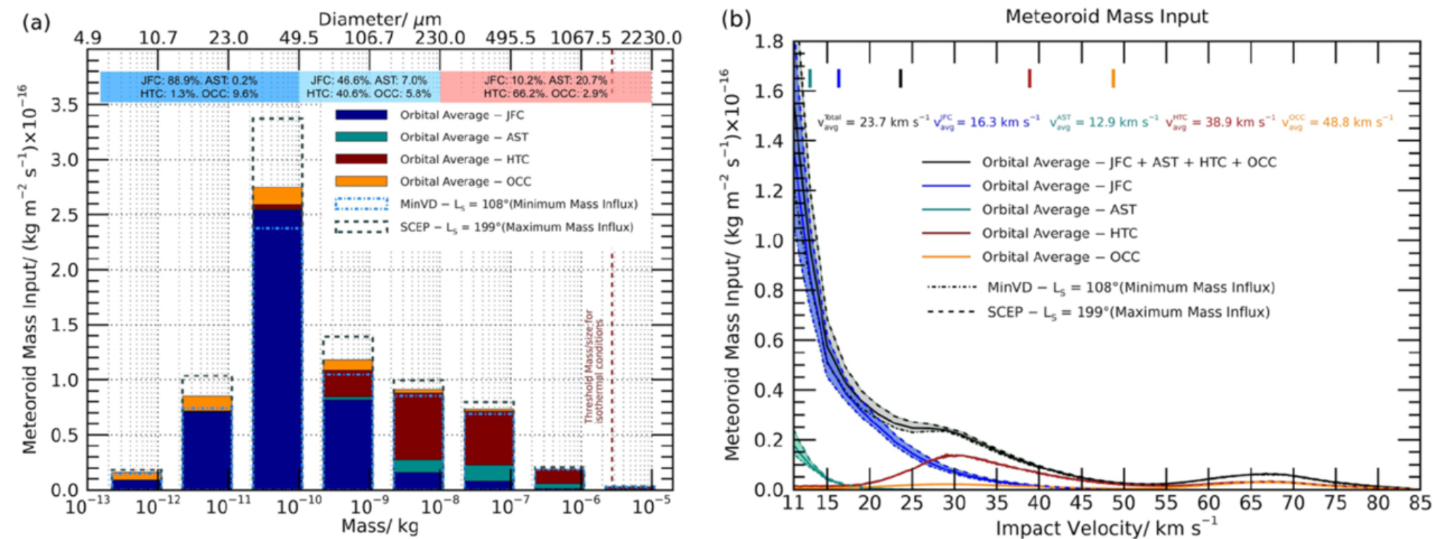
Figure 3. from Juan Diego Carrillo-Sánchez et al 2026 Planet. Sci. J. 7 doi:10.3847/PSJ/ae8257 https://dx.doi.org/10.3847/PSJ/ae8257 © 2026. The Author(s). Published by the American Astronomical Society.
