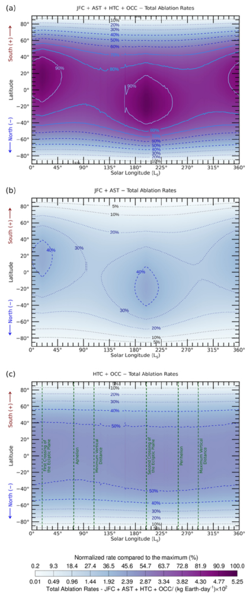
Figure 17. from Juan Diego Carrillo-Sánchez et al 2026 Planet. Sci. J. 7 doi:10.3847/PSJ/ae8257 https://dx.doi.org/10.3847/PSJ/ae8257 © 2026. The Author(s). Published by the American Astronomical Society.
