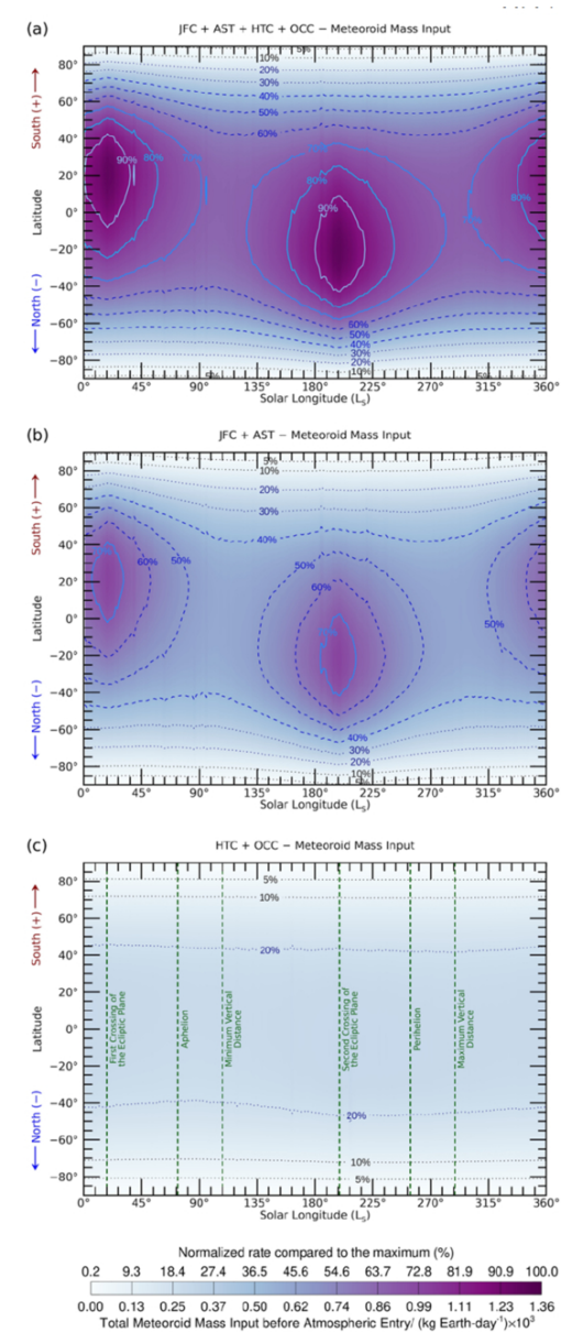
Figure 16. from Juan Diego Carrillo-Sánchez et al 2026 Planet. Sci. J. 7 doi:10.3847/PSJ/ae8257 https://dx.doi.org/10.3847/PSJ/ae8257 © 2026. The Author(s). Published by the American Astronomical Society.
