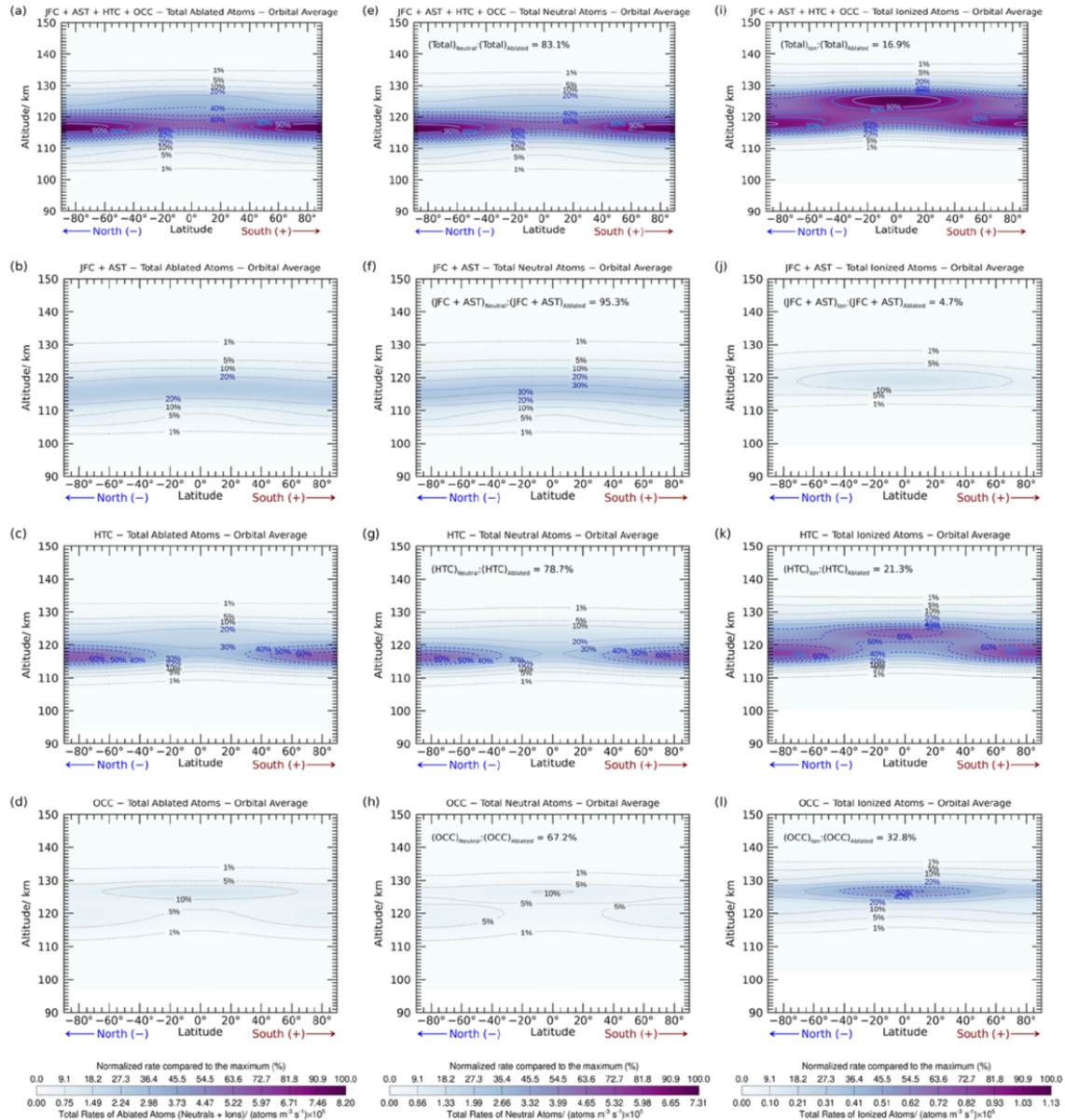
Figure 14. from Juan Diego Carrillo-Sánchez et al 2026 Planet. Sci. J. 7 doi:10.3847/PSJ/ae8257 https://dx.doi.org/10.3847/PSJ/ae8257 © 2026. The Author(s). Published by the American Astronomical Society.
