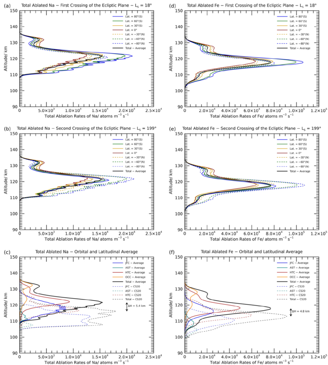
Figure 12. from Juan Diego Carrillo-Sánchez et al 2026 Planet. Sci. J. 7 doi:10.3847/PSJ/ae8257 https://dx.doi.org/10.3847/PSJ/ae8257 © 2026. The Author(s). Published by the American Astronomical Society.
