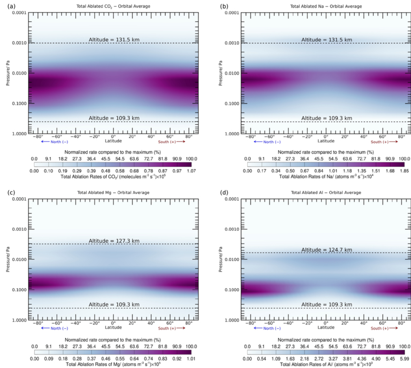
Figure 11. from Juan Diego Carrillo-Sánchez et al 2026 Planet. Sci. J. 7 doi:10.3847/PSJ/ae8257 https://dx.doi.org/10.3847/PSJ/ae8257 © 2026. The Author(s). Published by the American Astronomical Society.
