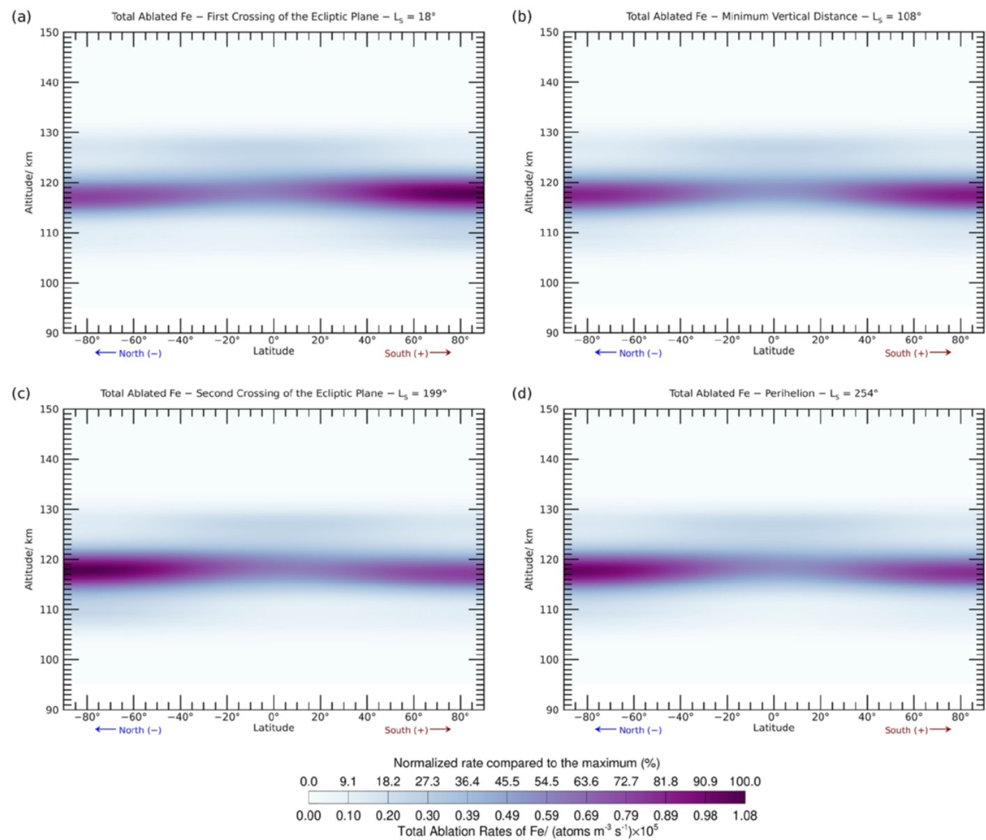
Figure 10. from Juan Diego Carrillo-Sánchez et al 2026 Planet. Sci. J. 7 doi:10.3847/PSJ/ae8257 https://dx.doi.org/10.3847/PSJ/ae8257 © 2026. The Author(s). Published by the American Astronomical Society.
