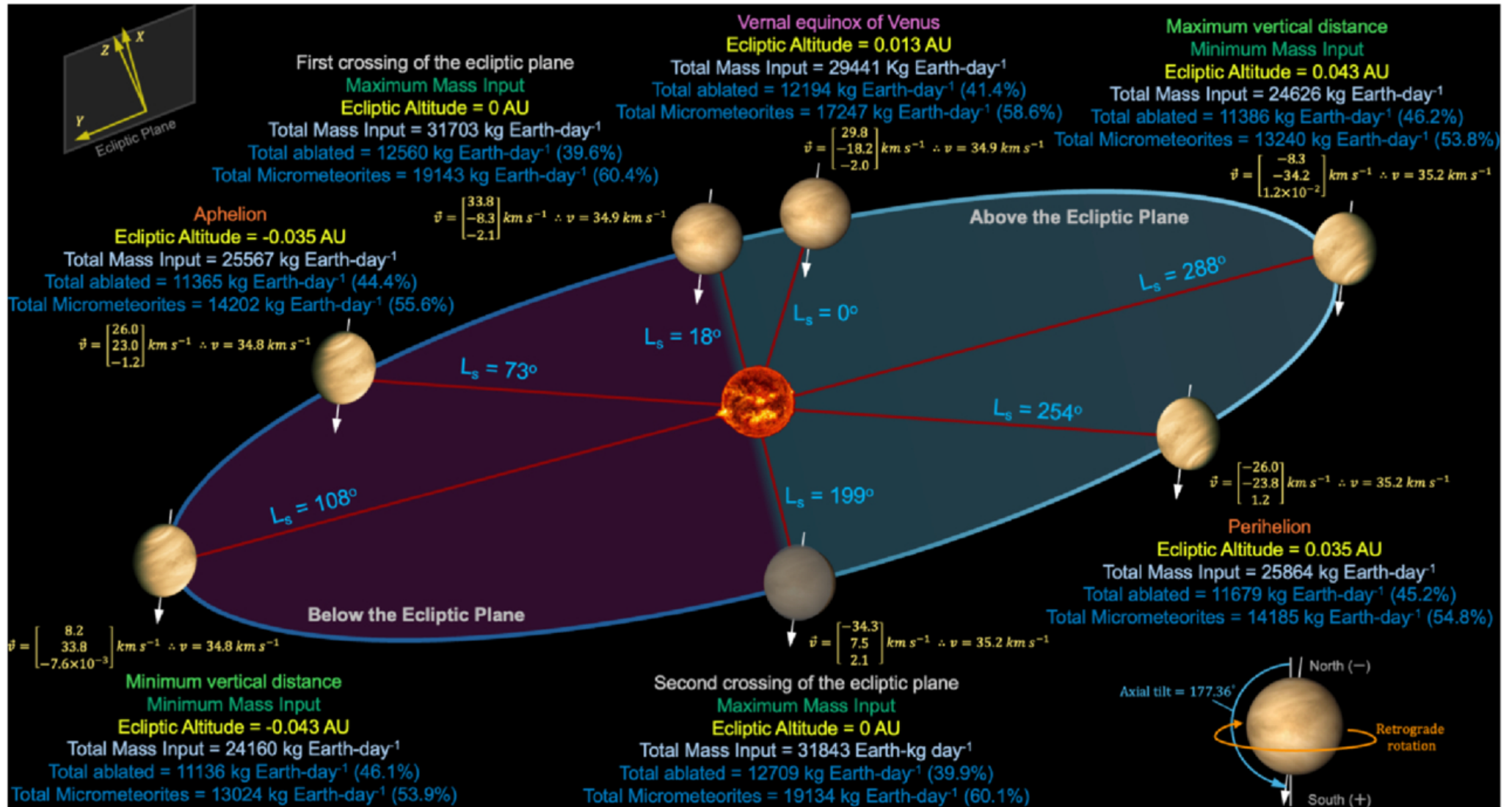
Figure 1. from Juan Diego Carrillo-Sánchez et al 2026 Planet. Sci. J. 7 doi:10.3847/PSJ/ae8257 https://dx.doi.org/10.3847/PSJ/ae8257 © 2026. The Author(s). Published by the American Astronomical Society.
