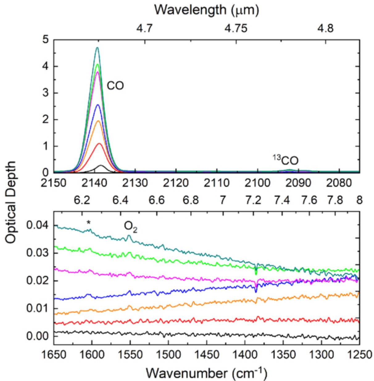
Figure 5. from William A. Burris et al 2026 Planet. Sci. J. 7 doi:10.3847/PSJ/ae81af https://dx.doi.org/10.3847/PSJ/ae81af © 2026. The Author(s). Published by the American Astronomical Society.
