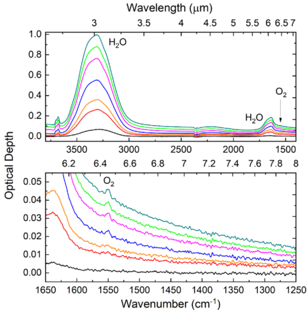
Figure 3. from William A. Burris et al 2026 Planet. Sci. J. 7 doi:10.3847/PSJ/ae81af https://dx.doi.org/10.3847/PSJ/ae81af © 2026. The Author(s). Published by the American Astronomical Society.
