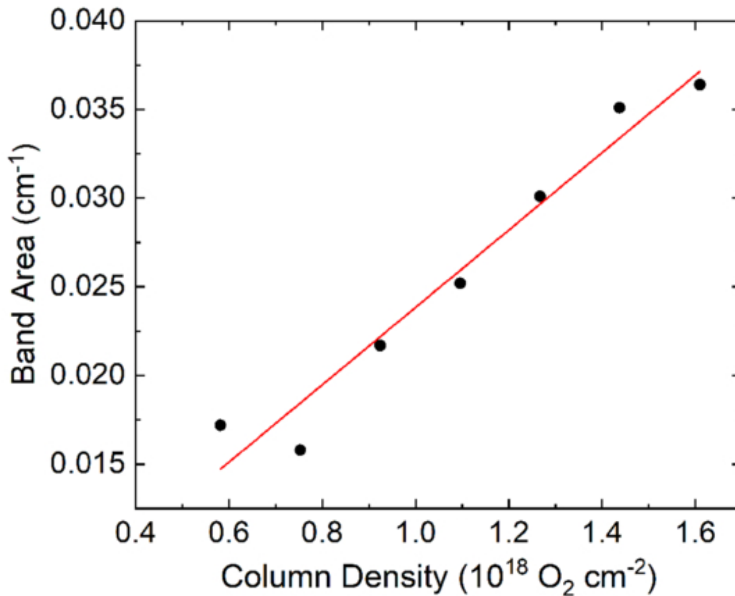
Figure 2. from William A. Burris et al 2026 Planet. Sci. J. 7 doi:10.3847/PSJ/ae81af https://dx.doi.org/10.3847/PSJ/ae81af © 2026. The Author(s). Published by the American Astronomical Society.
