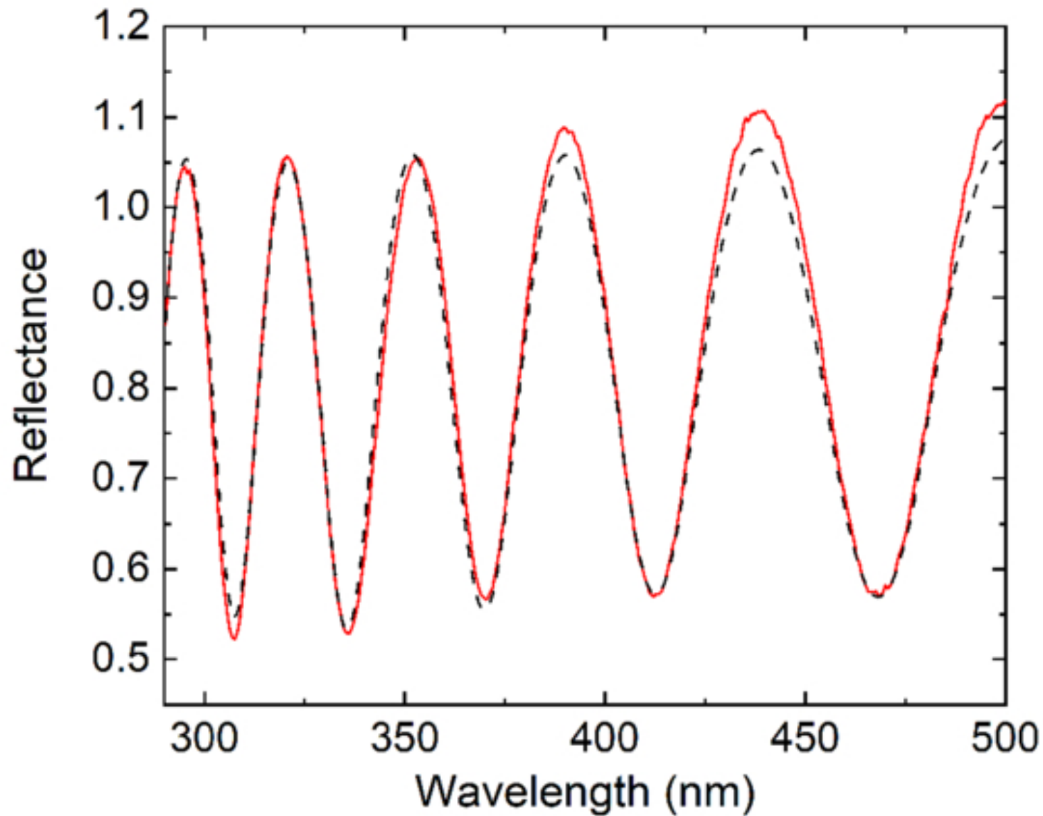
Figure 1. from William A. Burris et al 2026 Planet. Sci. J. 7 doi:10.3847/PSJ/ae81af https://dx.doi.org/10.3847/PSJ/ae81af © 2026. The Author(s). Published by the American Astronomical Society.
