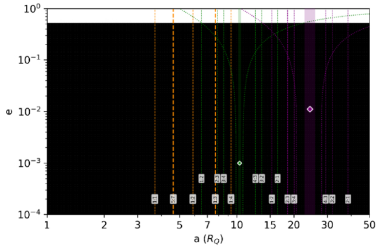
(a) 0
