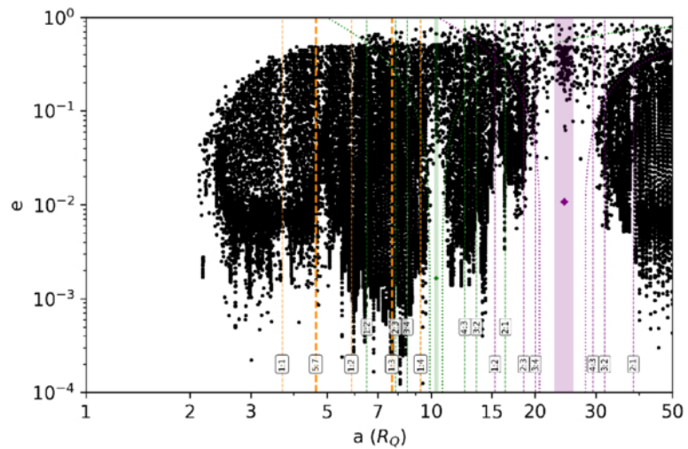
(c) 10^3 T_Q
