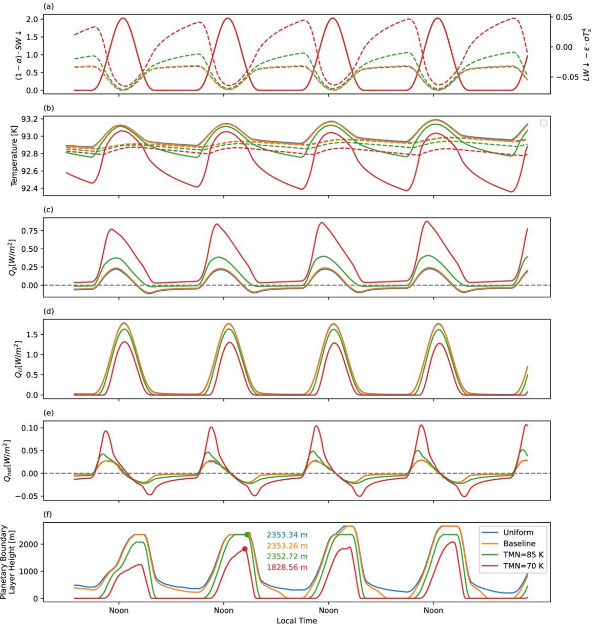
Figure A5. from Victoria L. Hartwick et al 2026 Planet. Sci. J. 7 doi:10.3847/PSJ/ae809d https://dx.doi.org/10.3847/PSJ/ae809d © 2026. The Author(s). Published by the American Astronomical Society.
