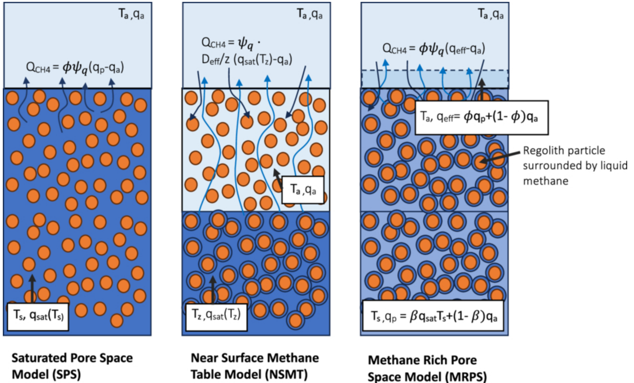
Figure 2. from Victoria L. Hartwick et al 2026 Planet. Sci. J. 7 doi:10.3847/PSJ/ae809d https://dx.doi.org/10.3847/PSJ/ae809d © 2026. The Author(s). Published by the American Astronomical Society.
