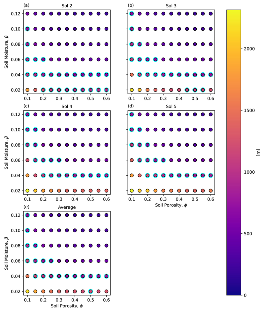
Figure 15. from Victoria L. Hartwick et al 2026 Planet. Sci. J. 7 doi:10.3847/PSJ/ae809d https://dx.doi.org/10.3847/PSJ/ae809d © 2026. The Author(s). Published by the American Astronomical Society.
