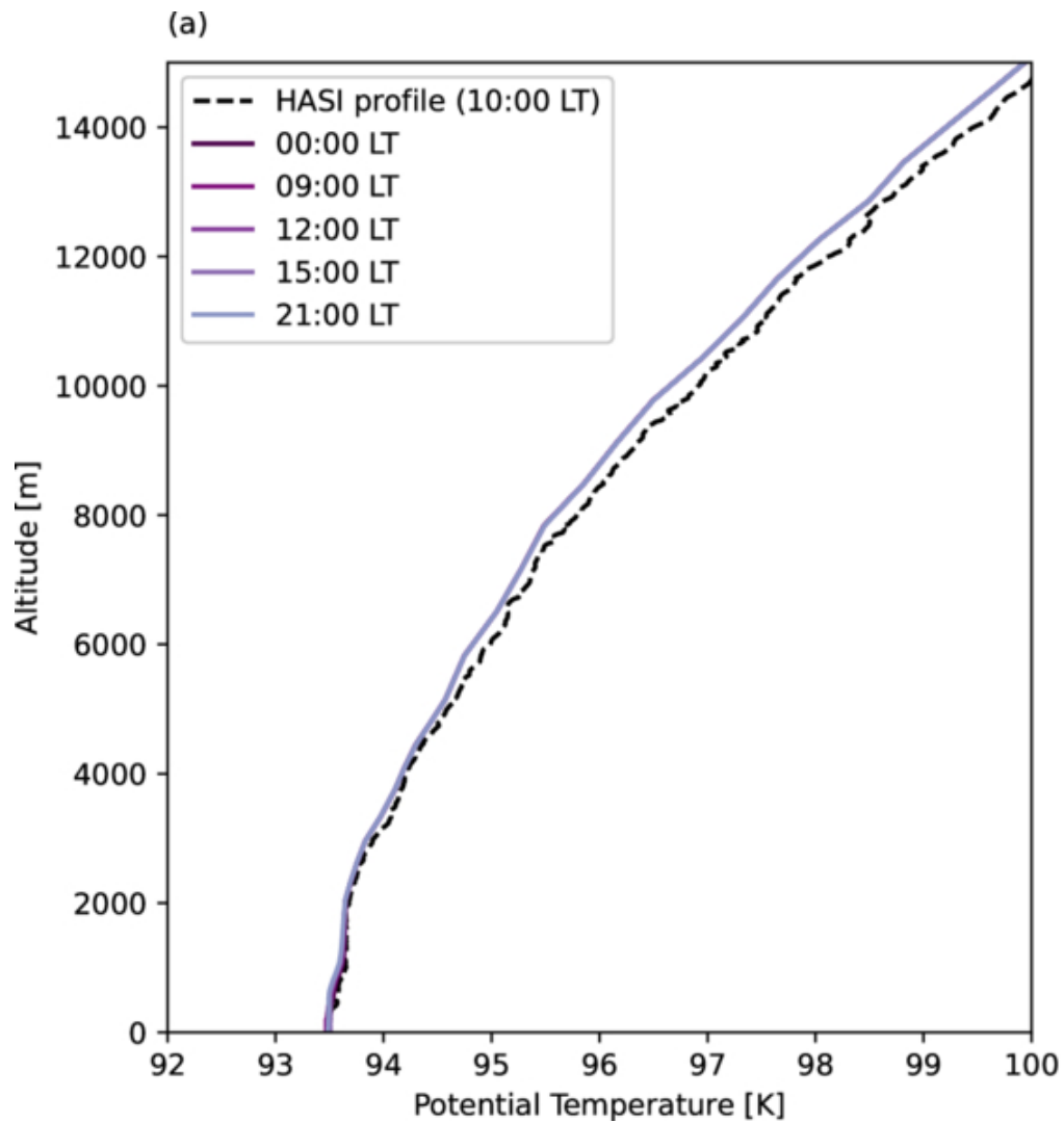
Figure 14. from Victoria L. Hartwick et al 2026 Planet. Sci. J. 7 doi:10.3847/PSJ/ae809d https://dx.doi.org/10.3847/PSJ/ae809d © 2026. The Author(s). Published by the American Astronomical Society.
