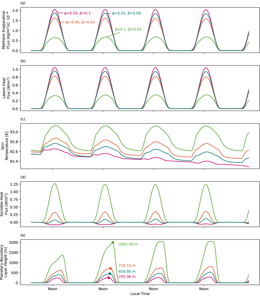
Figure 13. from Victoria L. Hartwick et al 2026 Planet. Sci. J. 7 doi:10.3847/PSJ/ae809d https://dx.doi.org/10.3847/PSJ/ae809d © 2026. The Author(s). Published by the American Astronomical Society.
