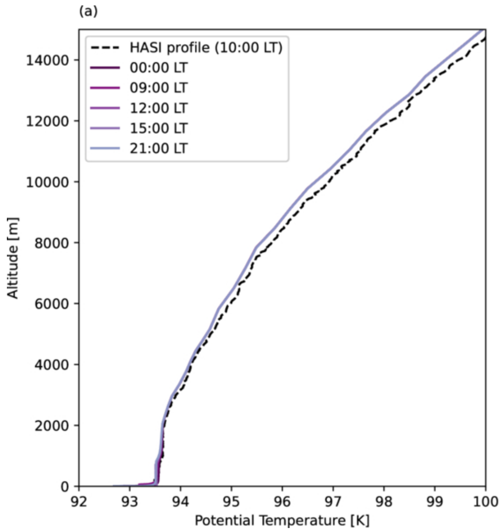
Figure 12. from Victoria L. Hartwick et al 2026 Planet. Sci. J. 7 doi:10.3847/PSJ/ae809d https://dx.doi.org/10.3847/PSJ/ae809d © 2026. The Author(s). Published by the American Astronomical Society.
