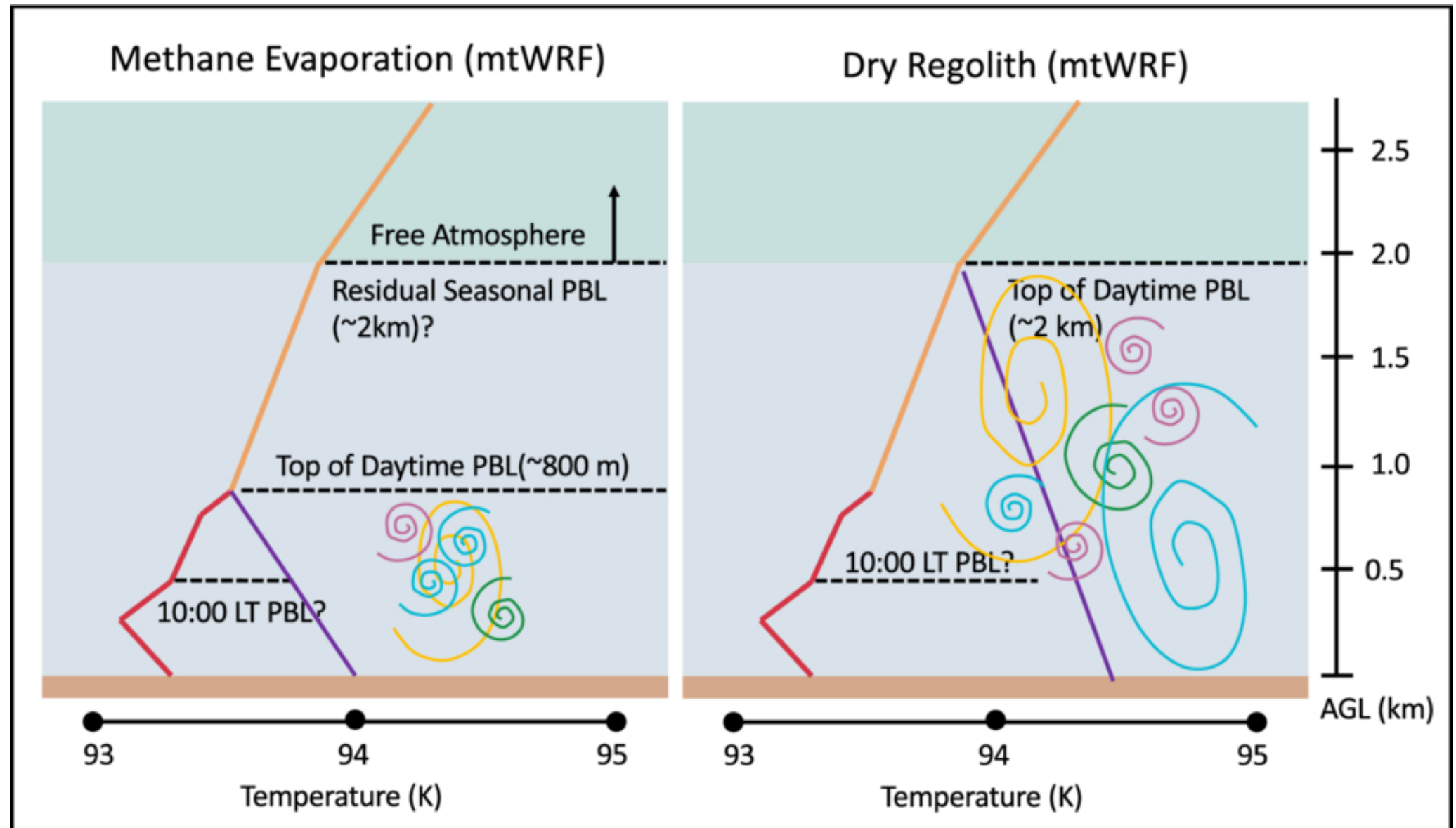
Figure 1. from Victoria L. Hartwick et al 2026 Planet. Sci. J. 7 doi:10.3847/PSJ/ae809d https://dx.doi.org/10.3847/PSJ/ae809d © 2026. The Author(s). Published by the American Astronomical Society.
