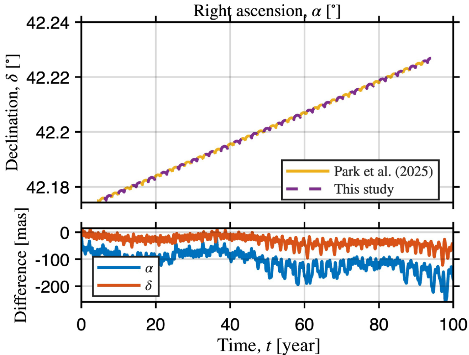
Figure 8. from Anton I. Ermakov 2026 Planet. Sci. J. 7 doi:10.3847/PSJ/ae7f03 https://dx.doi.org/10.3847/PSJ/ae7f03 © 2026. The Author(s). Published by the American Astronomical Society.
