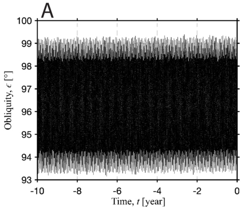
Figure 7. from Anton I. Ermakov 2026 Planet. Sci. J. 7 doi:10.3847/PSJ/ae7f03 https://dx.doi.org/10.3847/PSJ/ae7f03 © 2026. The Author(s). Published by the American Astronomical Society.
