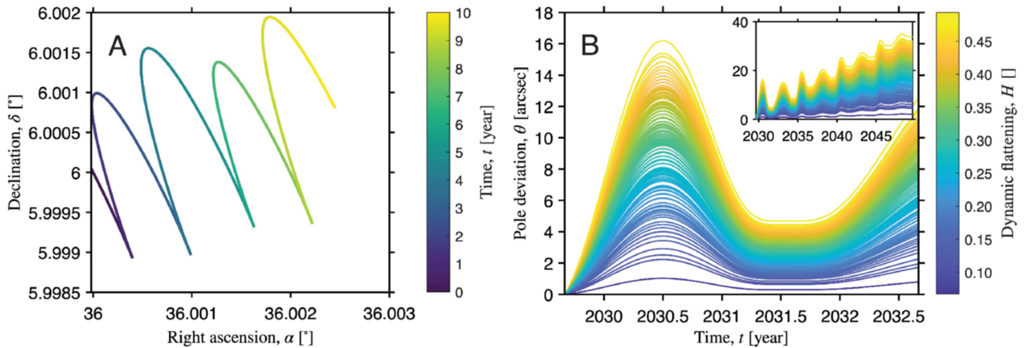
Figure 3. from Anton I. Ermakov 2026 Planet. Sci. J. 7 doi:10.3847/PSJ/ae7f03 https://dx.doi.org/10.3847/PSJ/ae7f03 © 2026. The Author(s). Published by the American Astronomical Society.
