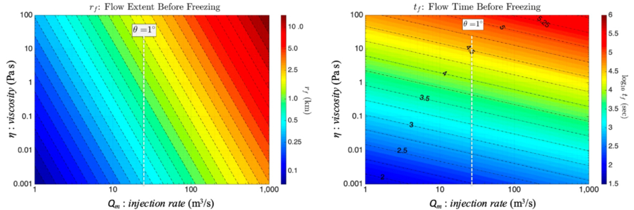
Figure 3. from S. A. Stern et al 2026 Planet. Sci. J. 7 doi:10.3847/PSJ/ae7e85 https://dx.doi.org/10.3847/PSJ/ae7e85 © 2026. The Author(s). Published by the American Astronomical Society.
