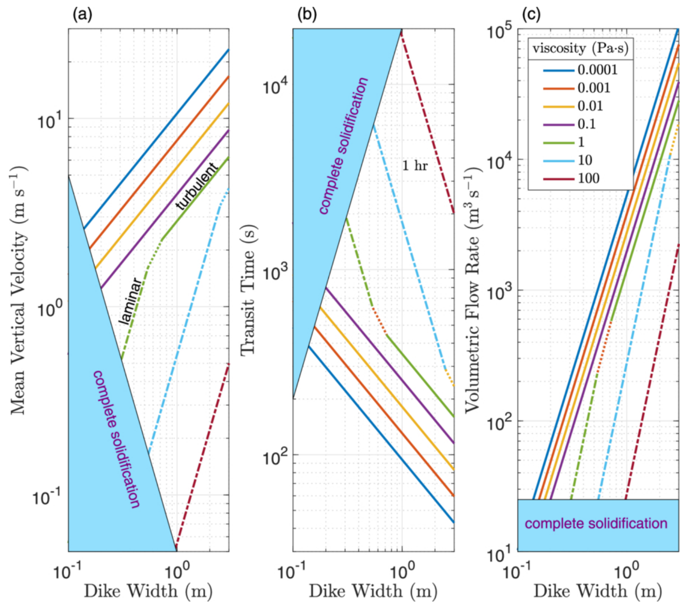
Figure D3. from S. A. Stern et al 2026 Planet. Sci. J. 7 doi:10.3847/PSJ/ae7e85 https://dx.doi.org/10.3847/PSJ/ae7e85 © 2026. The Author(s). Published by the American Astronomical Society.
