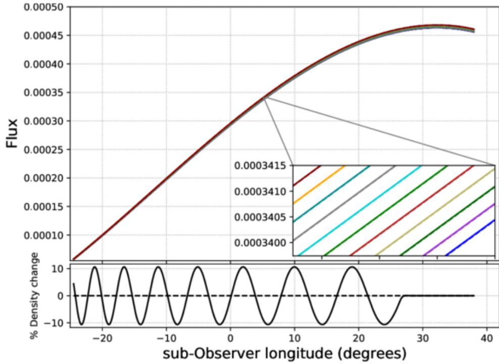
Figure 8. from Gourav Mahapatra et al 2026 Planet. Sci. J. 7 doi:10.3847/PSJ/ae7e6f https://dx.doi.org/10.3847/PSJ/ae7e6f © 2026. The Author(s). Published by the American Astronomical Society.
