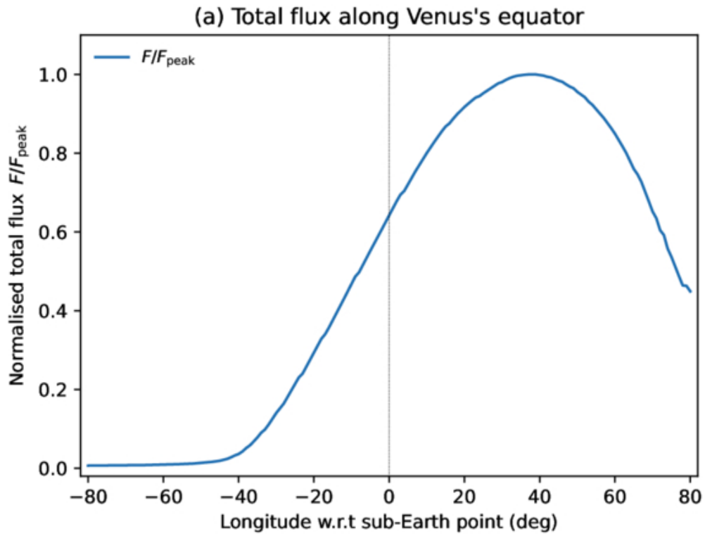
Figure 2. from Gourav Mahapatra et al 2026 Planet. Sci. J. 7 doi:10.3847/PSJ/ae7e6f https://dx.doi.org/10.3847/PSJ/ae7e6f © 2026. The Author(s). Published by the American Astronomical Society.
