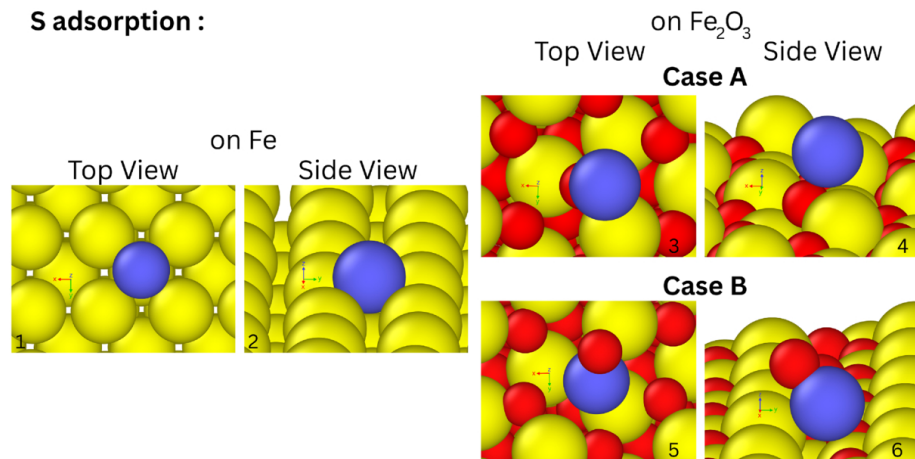
Figure 2. from S. Verkercke et al 2026 Planet. Sci. J. 7 doi:10.3847/PSJ/ae7d1d https://dx.doi.org/10.3847/PSJ/ae7d1d © 2026. The Author(s). Published by the American Astronomical Society.
