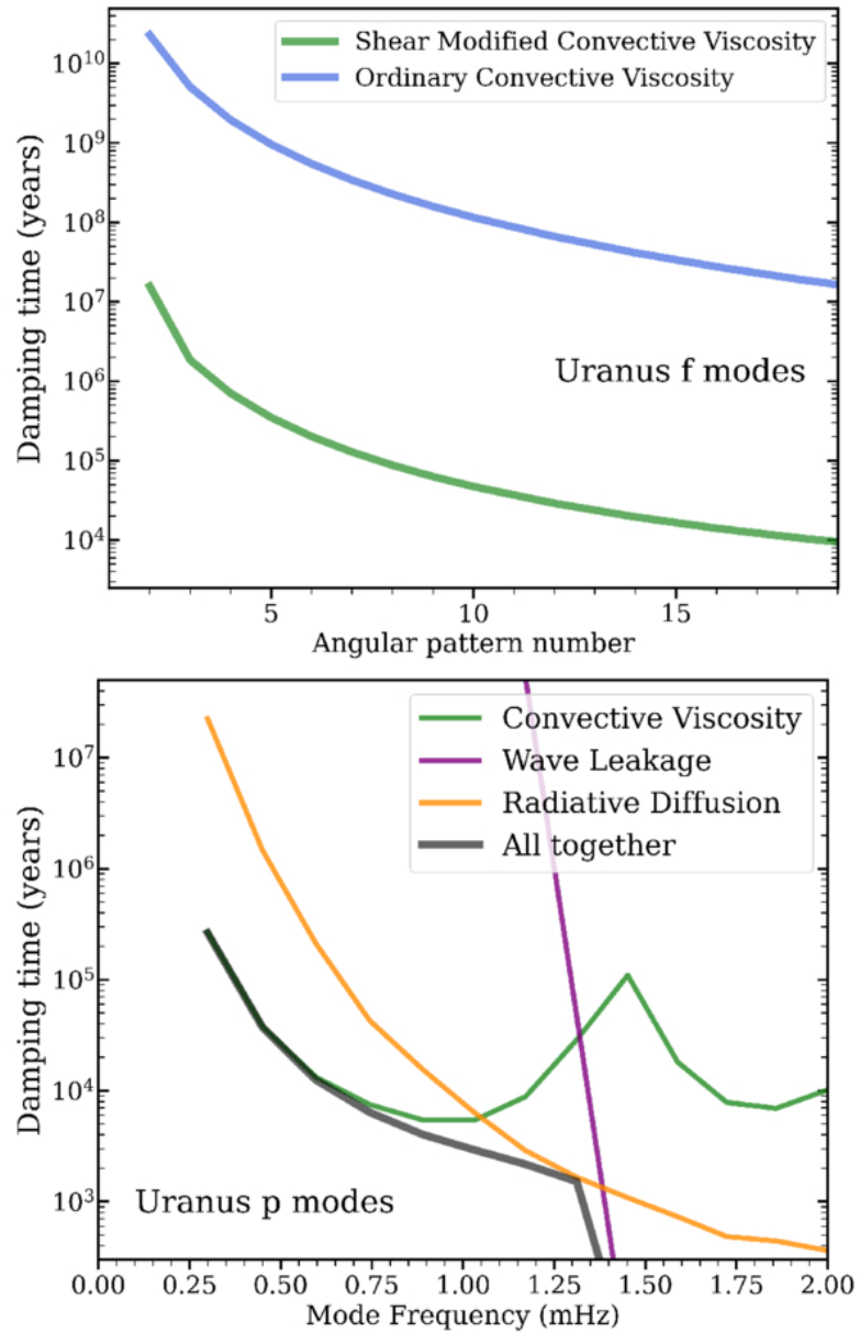
Figure 6. from Jim Fuller et al 2026 Planet. Sci. J. 7 doi:10.3847/PSJ/ae7bf4 https://dx.doi.org/10.3847/PSJ/ae7bf4 © 2026. The Author(s). Published by the American Astronomical Society.
