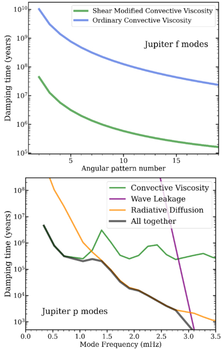
Figure 5. from Jim Fuller et al 2026 Planet. Sci. J. 7 doi:10.3847/PSJ/ae7bf4 https://dx.doi.org/10.3847/PSJ/ae7bf4 © 2026. The Author(s). Published by the American Astronomical Society.
