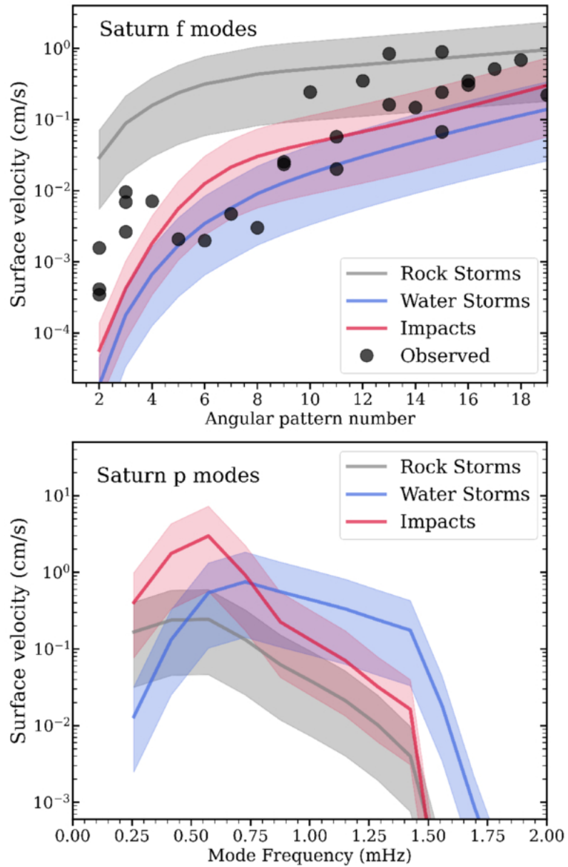
Figure 10. from Jim Fuller et al 2026 Planet. Sci. J. 7 doi:10.3847/PSJ/ae7bf4 https://dx.doi.org/10.3847/PSJ/ae7bf4 © 2026. The Author(s). Published by the American Astronomical Society.
