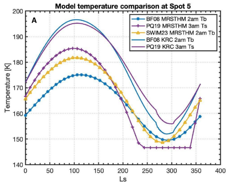
Figure 7. from Hanna G. Sizemore et al 2026 Planet. Sci. J. 7 doi:10.3847/PSJ/ae7b38 https://dx.doi.org/10.3847/PSJ/ae7b38 © 2026. The Author(s). Published by the American Astronomical Society.
