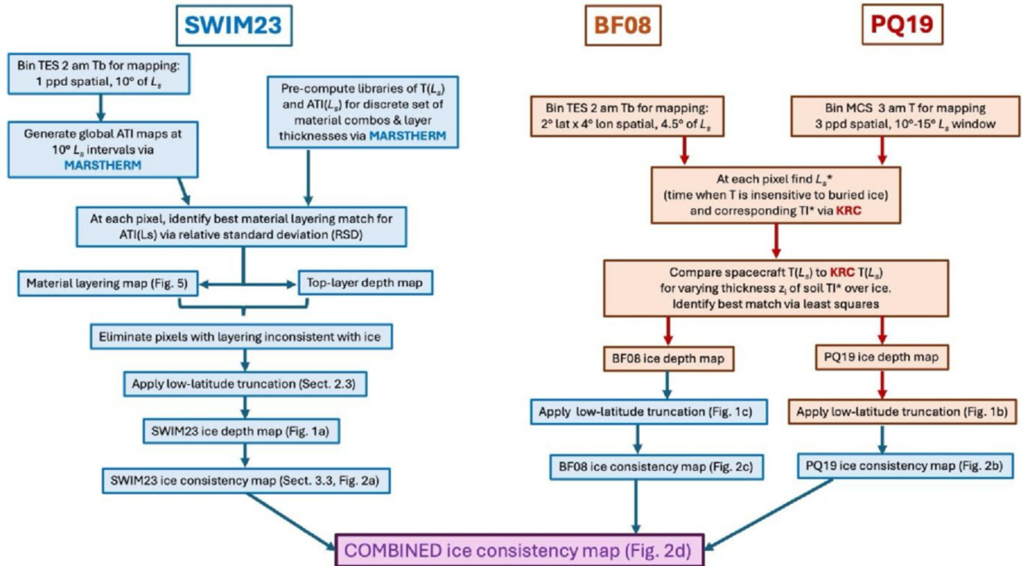
Figure 3. from Hanna G. Sizemore et al 2026 Planet. Sci. J. 7 doi:10.3847/PSJ/ae7b38 https://dx.doi.org/10.3847/PSJ/ae7b38 © 2026. The Author(s). Published by the American Astronomical Society.
