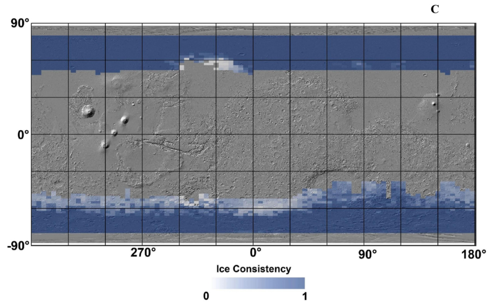
Figure 2. from Hanna G. Sizemore et al 2026 Planet. Sci. J. 7 doi:10.3847/PSJ/ae7b38 https://dx.doi.org/10.3847/PSJ/ae7b38 © 2026. The Author(s). Published by the American Astronomical Society.
