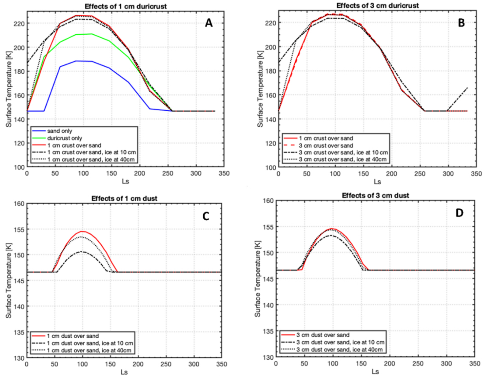
Figure 14. from Hanna G. Sizemore et al 2026 Planet. Sci. J. 7 doi:10.3847/PSJ/ae7b38 https://dx.doi.org/10.3847/PSJ/ae7b38 © 2026. The Author(s). Published by the American Astronomical Society.
