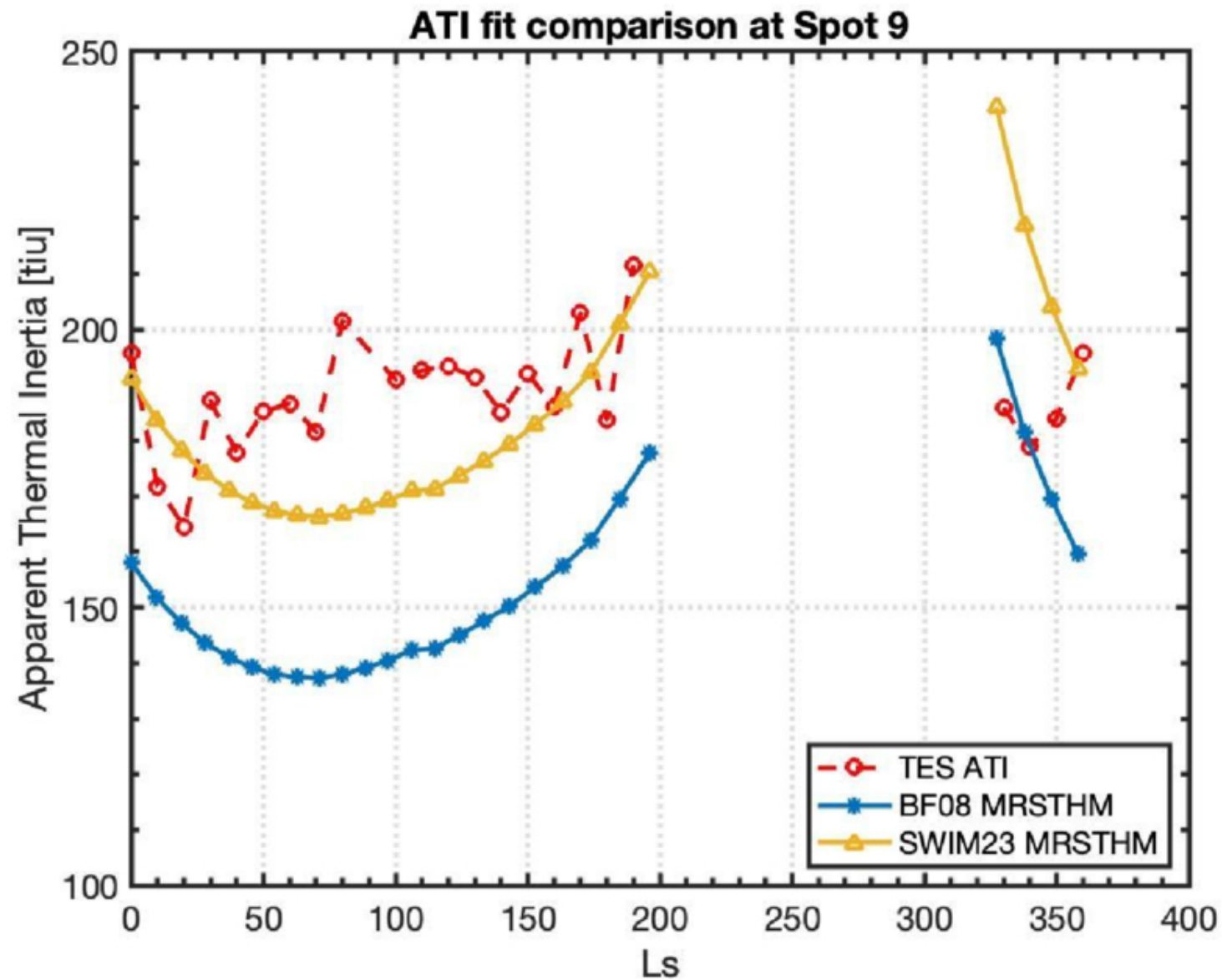
Figure 11. from Hanna G. Sizemore et al 2026 Planet. Sci. J. 7 doi:10.3847/PSJ/ae7b38 https://dx.doi.org/10.3847/PSJ/ae7b38 © 2026. The Author(s). Published by the American Astronomical Society.
