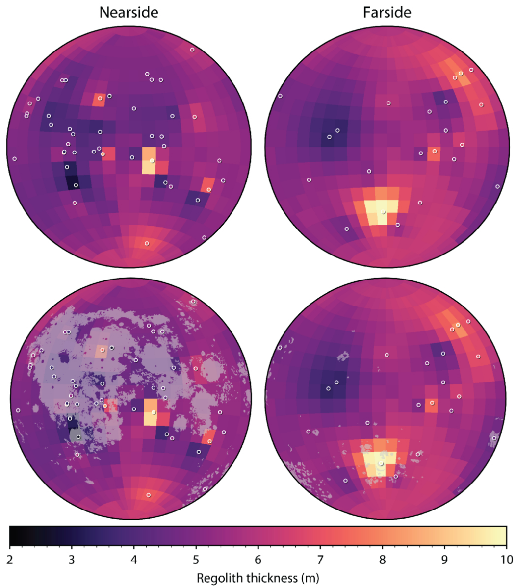
Figure 7. from Andrea Rajši et al 2026 Planet. Sci. J. 7 doi:10.3847/PSJ/ae7a6f https://dx.doi.org/10.3847/PSJ/ae7a6f © 2026. The Author(s). Published by the American Astronomical Society.
