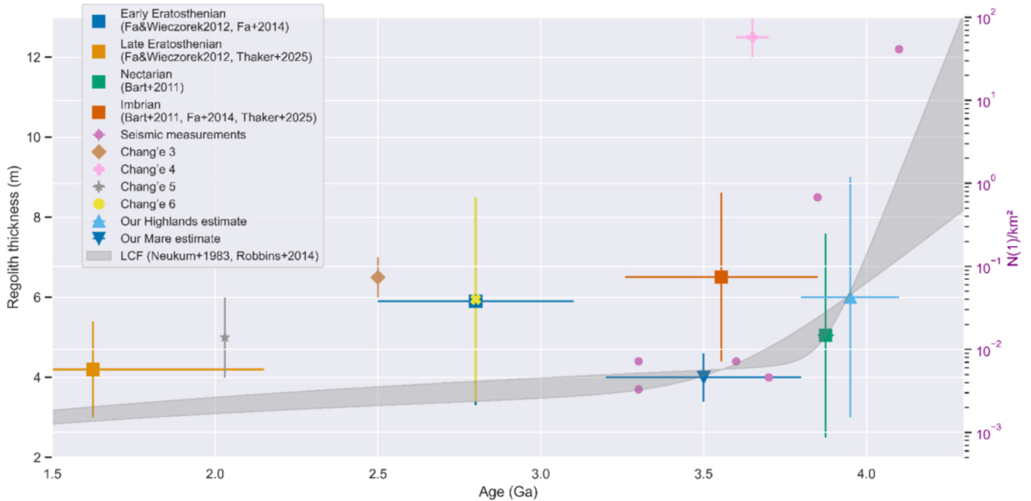
Figure 6. from Andrea Rajši et al 2026 Planet. Sci. J. 7 doi:10.3847/PSJ/ae7a6f https://dx.doi.org/10.3847/PSJ/ae7a6f © 2026. The Author(s). Published by the American Astronomical Society.
