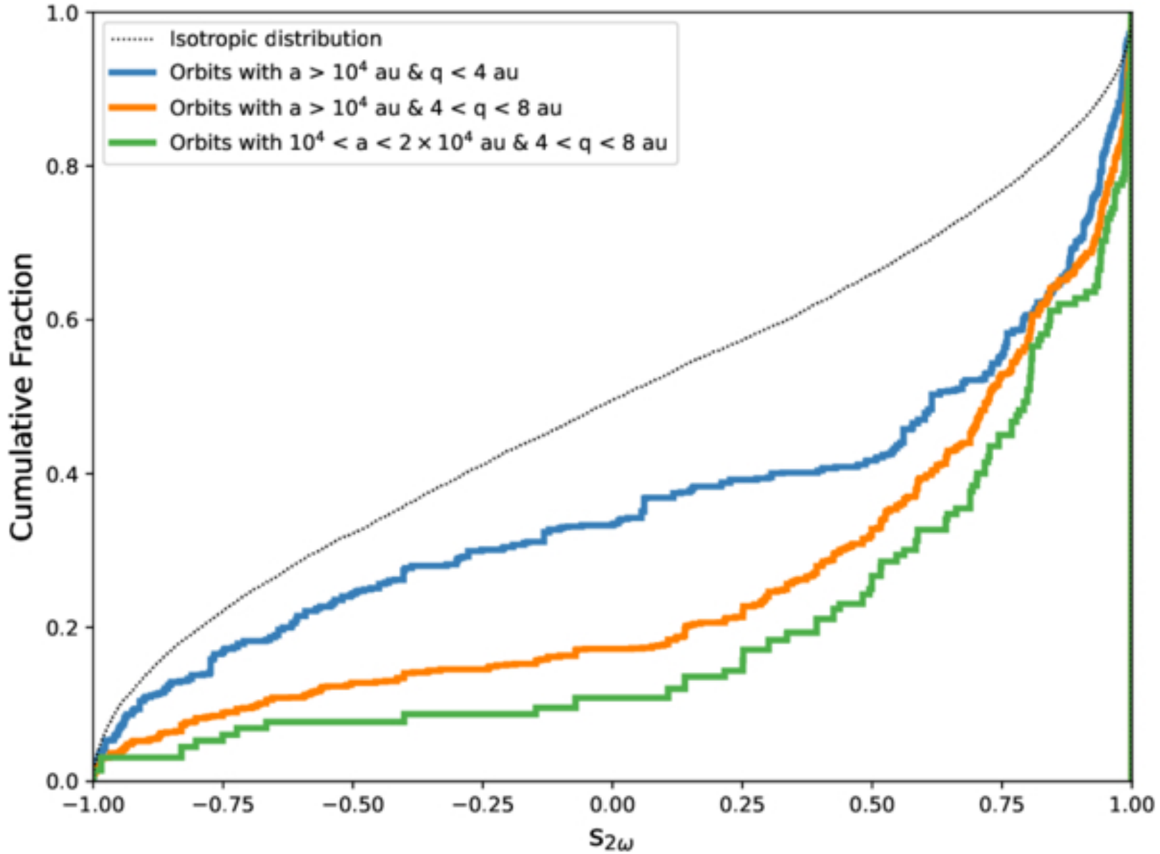
Figure 3. from Nathan A. Kaib and Sean N. Raymond 2026 Planet. Sci. J. 7 doi:10.3847/PSJ/ae7a65 https://dx.doi.org/10.3847/PSJ/ae7a65 © 2026. The Author(s). Published by the American Astronomical Society.
