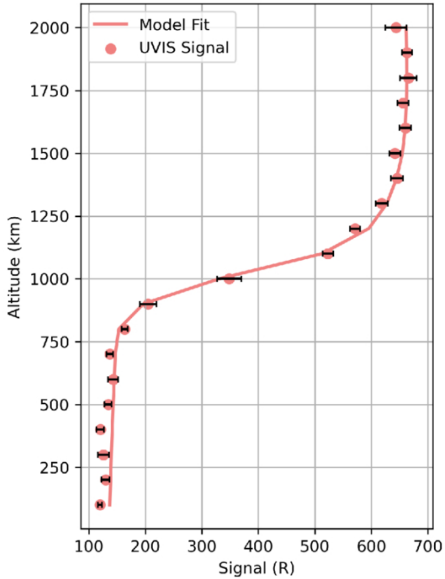
Figure 7. from Devin Hoover et al 2026 Planet. Sci. J. 7 doi:10.3847/PSJ/ae7a46 https://dx.doi.org/10.3847/PSJ/ae7a46 © 2026. The Author(s). Published by the American Astronomical Society.
