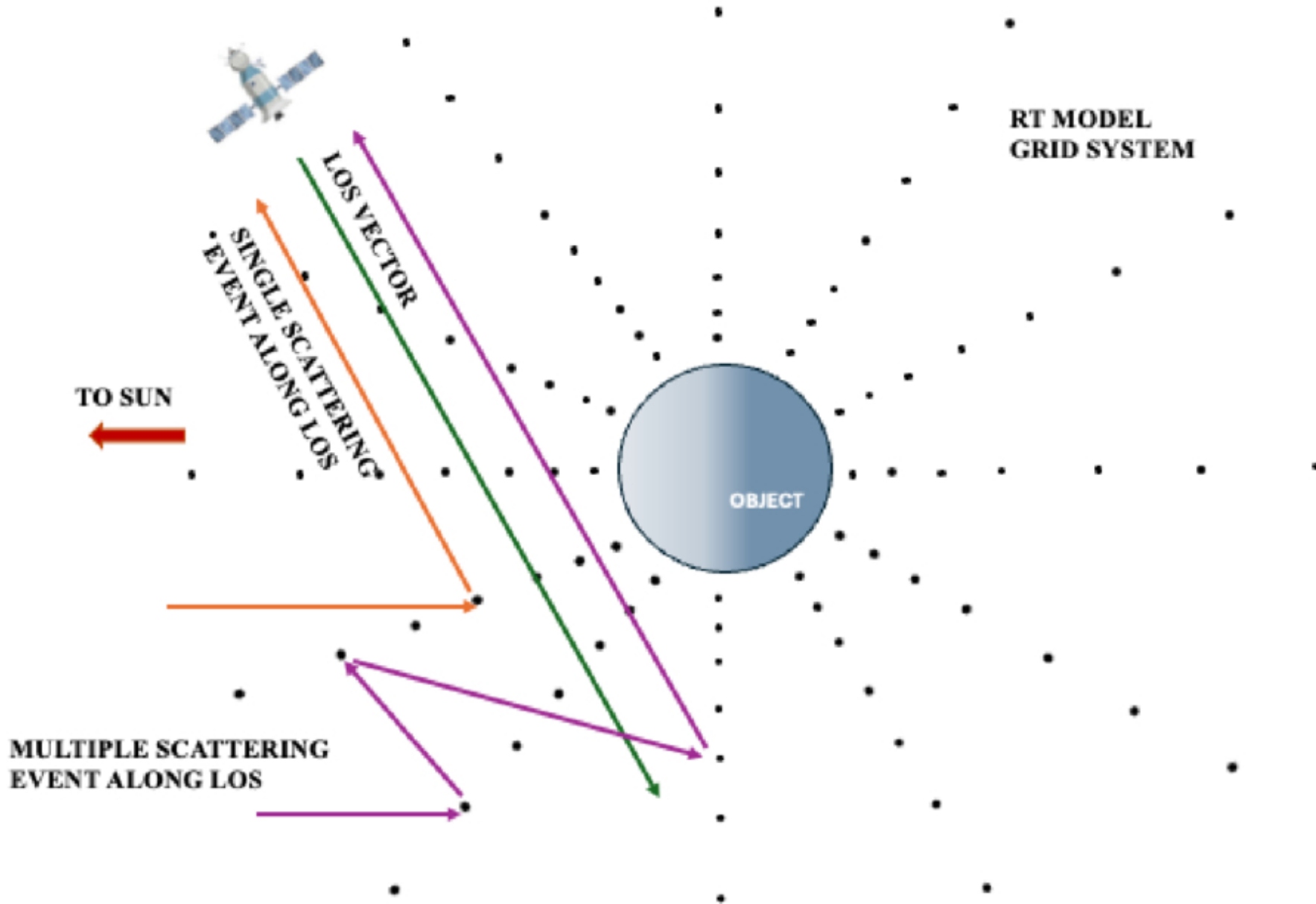
Figure 6. from Devin Hoover et al 2026 Planet. Sci. J. 7 doi:10.3847/PSJ/ae7a46 https://dx.doi.org/10.3847/PSJ/ae7a46 © 2026. The Author(s). Published by the American Astronomical Society.
