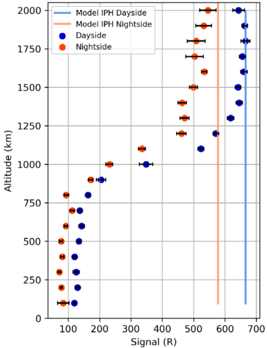
Figure 3. from Devin Hoover et al 2026 Planet. Sci. J. 7 doi:10.3847/PSJ/ae7a46 https://dx.doi.org/10.3847/PSJ/ae7a46 © 2026. The Author(s). Published by the American Astronomical Society.
