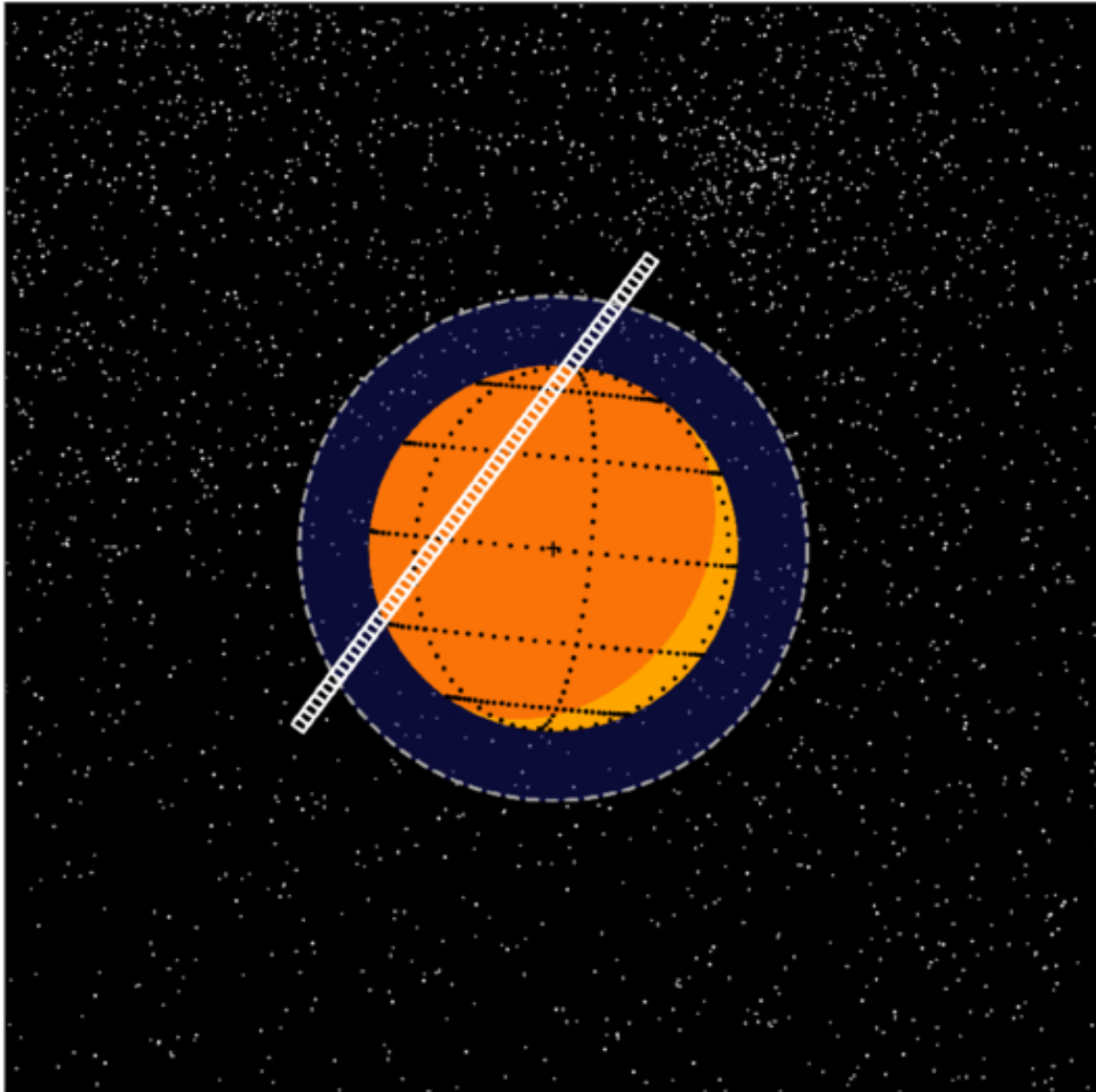
Figure 1. from Devin Hoover et al 2026 Planet. Sci. J. 7 doi:10.3847/PSJ/ae7a46 https://dx.doi.org/10.3847/PSJ/ae7a46 © 2026. The Author(s). Published by the American Astronomical Society.
