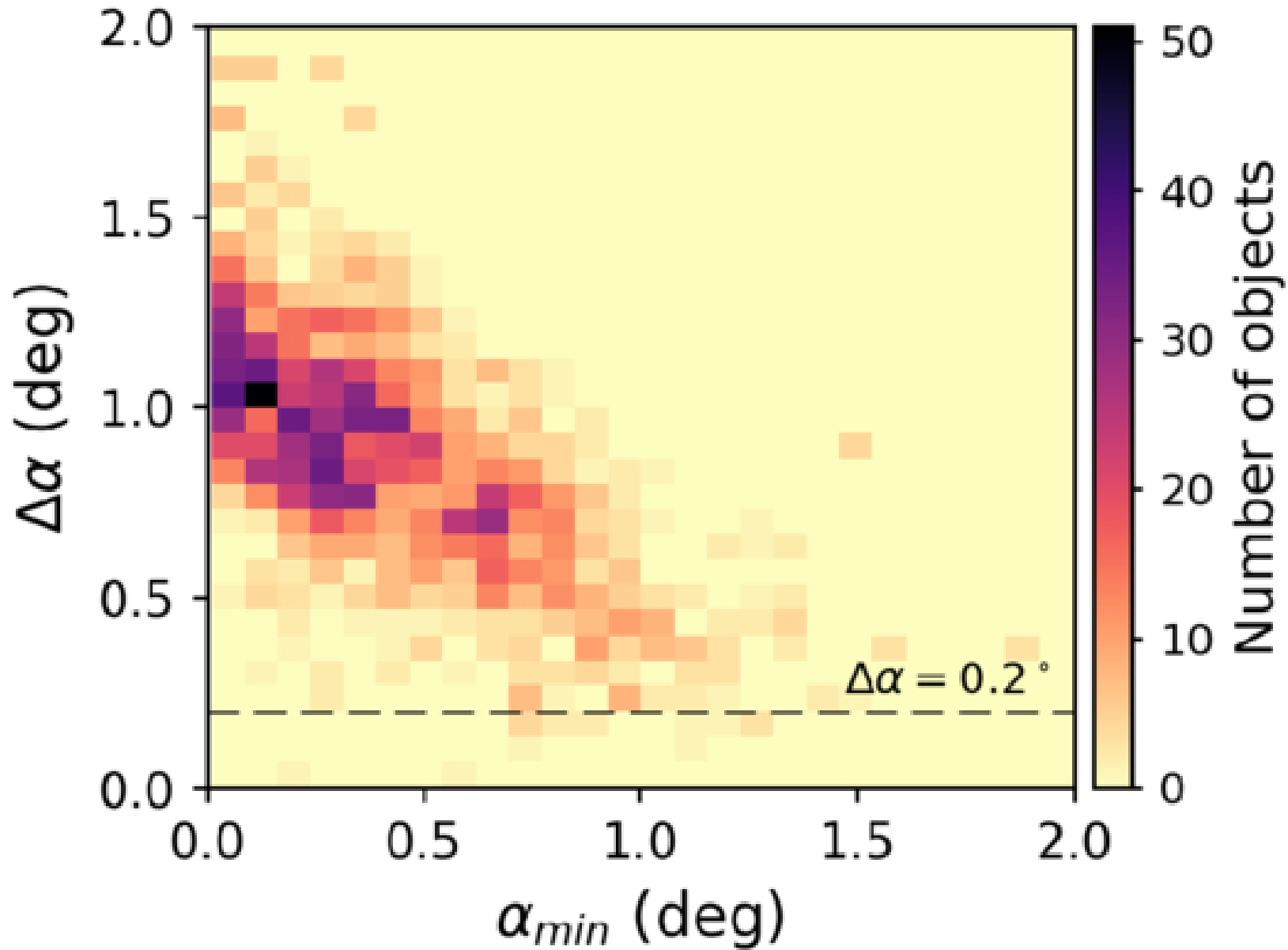
Figure 2. from Milagros Colazo and Alvaro Alvarez-Candal 2026 Planet. Sci. J. 7 doi:10.3847/PSJ/ae7a3f https://dx.doi.org/10.3847/PSJ/ae7a3f © 2026. The Author(s). Published by the American Astronomical Society.
