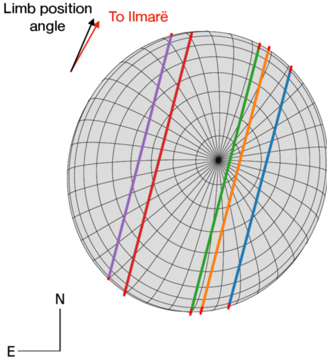
Figure 4. from Benjamin Proudfoot et al 2026 Planet. Sci. J. 7 doi:10.3847/PSJ/ae77fa https://dx.doi.org/10.3847/PSJ/ae77fa © 2026. The Author(s). Published by the American Astronomical Society.
