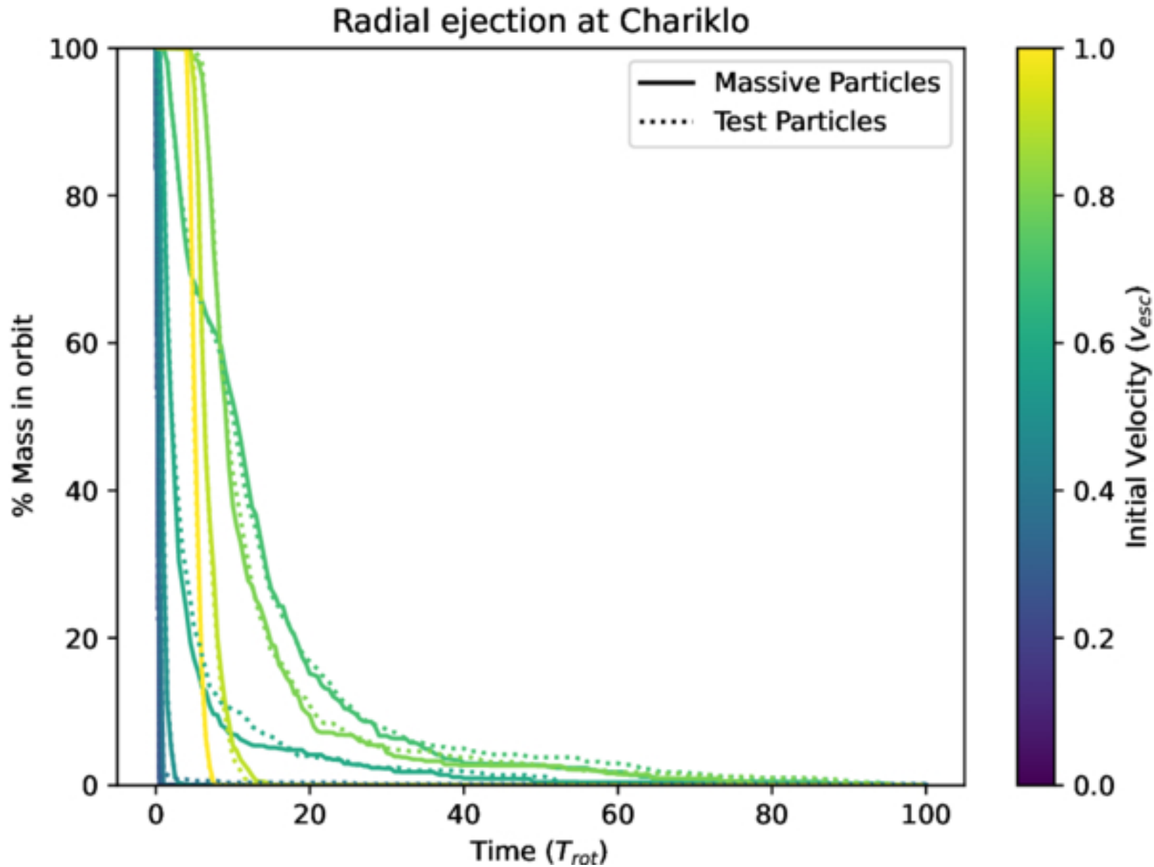
Figure 5. from Kaustub P. Anand et al 2026 Planet. Sci. J. 7 doi:10.3847/PSJ/ae7724 https://dx.doi.org/10.3847/PSJ/ae7724 © 2026. The Author(s). Published by the American Astronomical Society.
