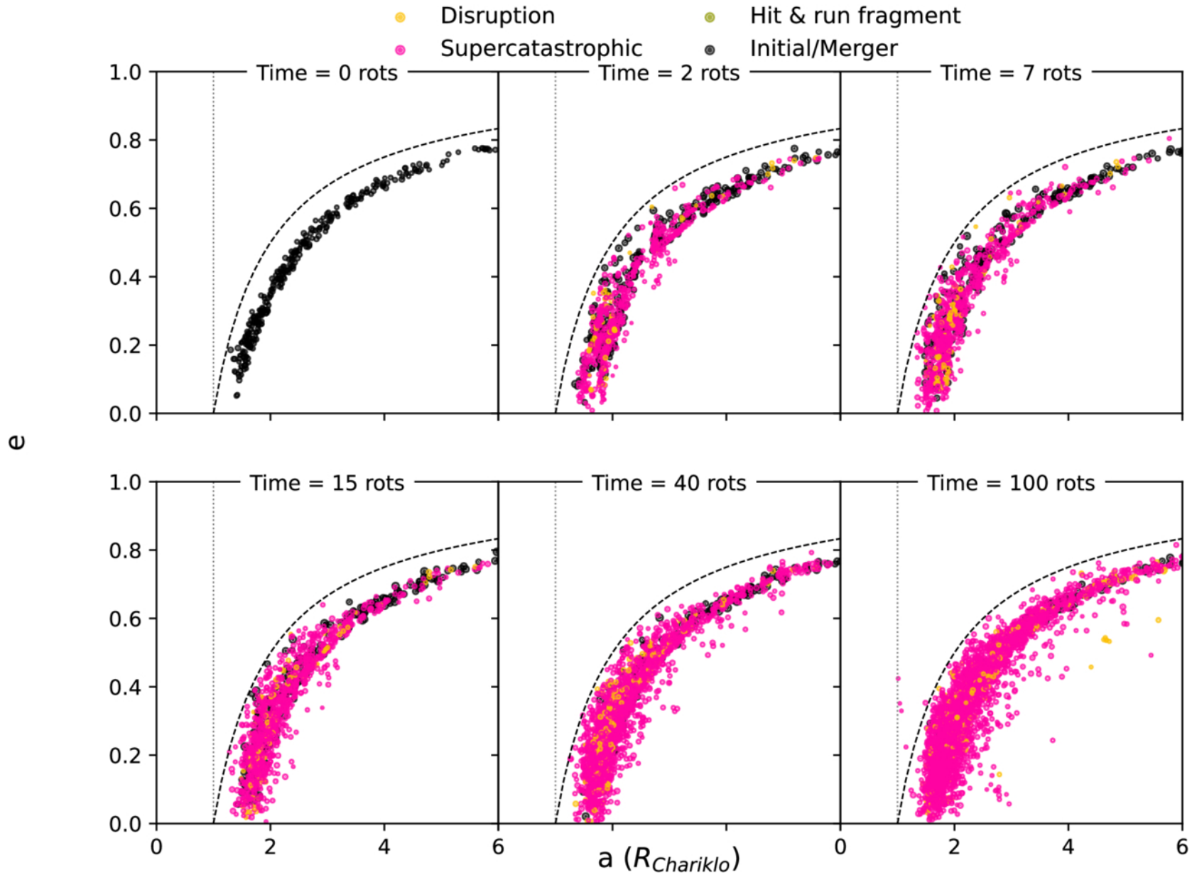
Figure 4. from Kaustub P. Anand et al 2026 Planet. Sci. J. 7 doi:10.3847/PSJ/ae7724 https://dx.doi.org/10.3847/PSJ/ae7724 © 2026. The Author(s). Published by the American Astronomical Society.
