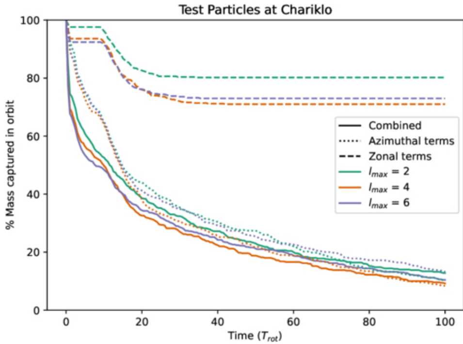
Figure 11. from Kaustub P. Anand et al 2026 Planet. Sci. J. 7 doi:10.3847/PSJ/ae7724 https://dx.doi.org/10.3847/PSJ/ae7724 © 2026. The Author(s). Published by the American Astronomical Society.
