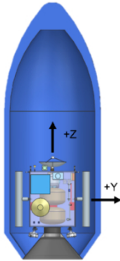
(a) Gelato in its stowed, launch configuration inside a high performance 5 m ELV payload fairing.
